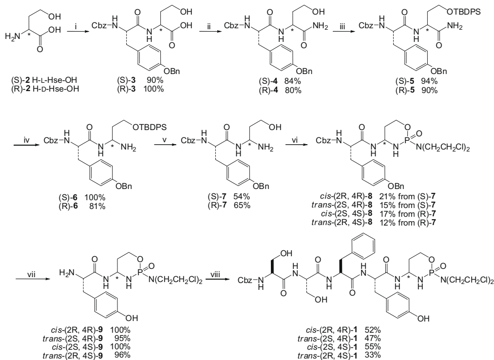
Scheme 1. Synthesis of diastereomers of Cbz-Ser-Ser-Tyr-Phe-NH-CPA ( 1 ) from D- or L-homoserine. Reagents and conditions: (i) Cbz-Tyr(Bn)-OSu, 1 M KHCO 3 , THF, rt; (ii) HOBt, EDC, THF, rt, then satd NH 3 (aq); (iii) TBDPS-Cl, imidazole, DMF, rt; (iv) BTI, CH 3 CN/H 2 O (1/1), rt; (v) TBAF, THF, rt; (vi) n -BuLi, HMAP, THF, -70 °C for 2 h, then Cl 2 PON(CH 2 CH 2 Cl) 2 , TEA, rt, 48 h; (vii) H 2 , Pd/C (10%), MeOH, rt; (viii) Cbz-Ser-Ser-Phe-OSu, DIEA, DME (dimethoxyethane).
