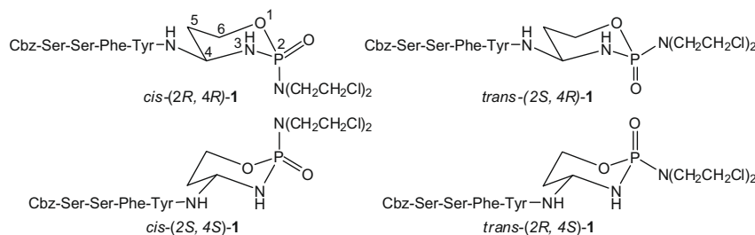
Figure 1. Four stereoisomers of Cbz-Ser-Ser-Phe-Tyr-NH-CPA ( 1 ).
